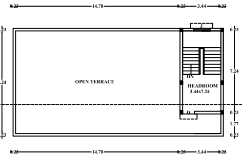
FLOOR-TERRACE
