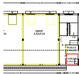
FLOOR-GROUND
