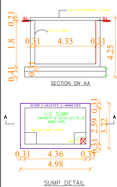
SUMP DETAIL
