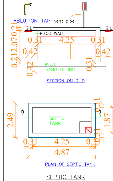
SEPTIC TANK
