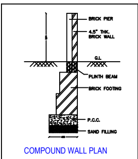
COMPOUND WALL PLAN
