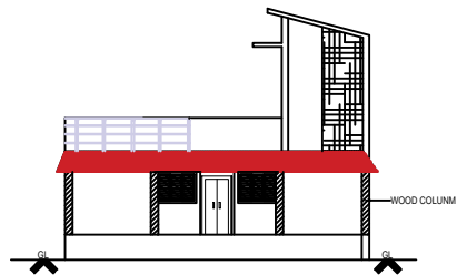
ELEVATION VIEW
