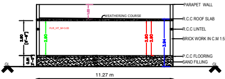
SECTION VIEW L-L
