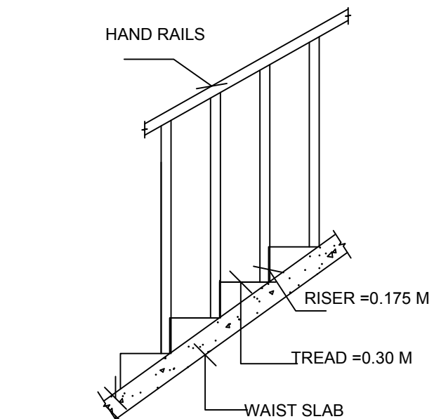
0.12 STAIR CASE DETAILS
