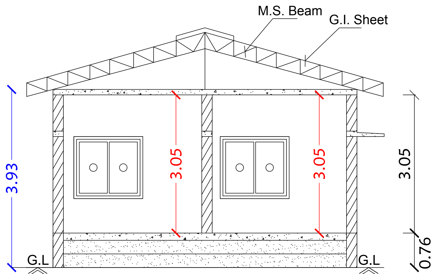
Section on-"AA"
