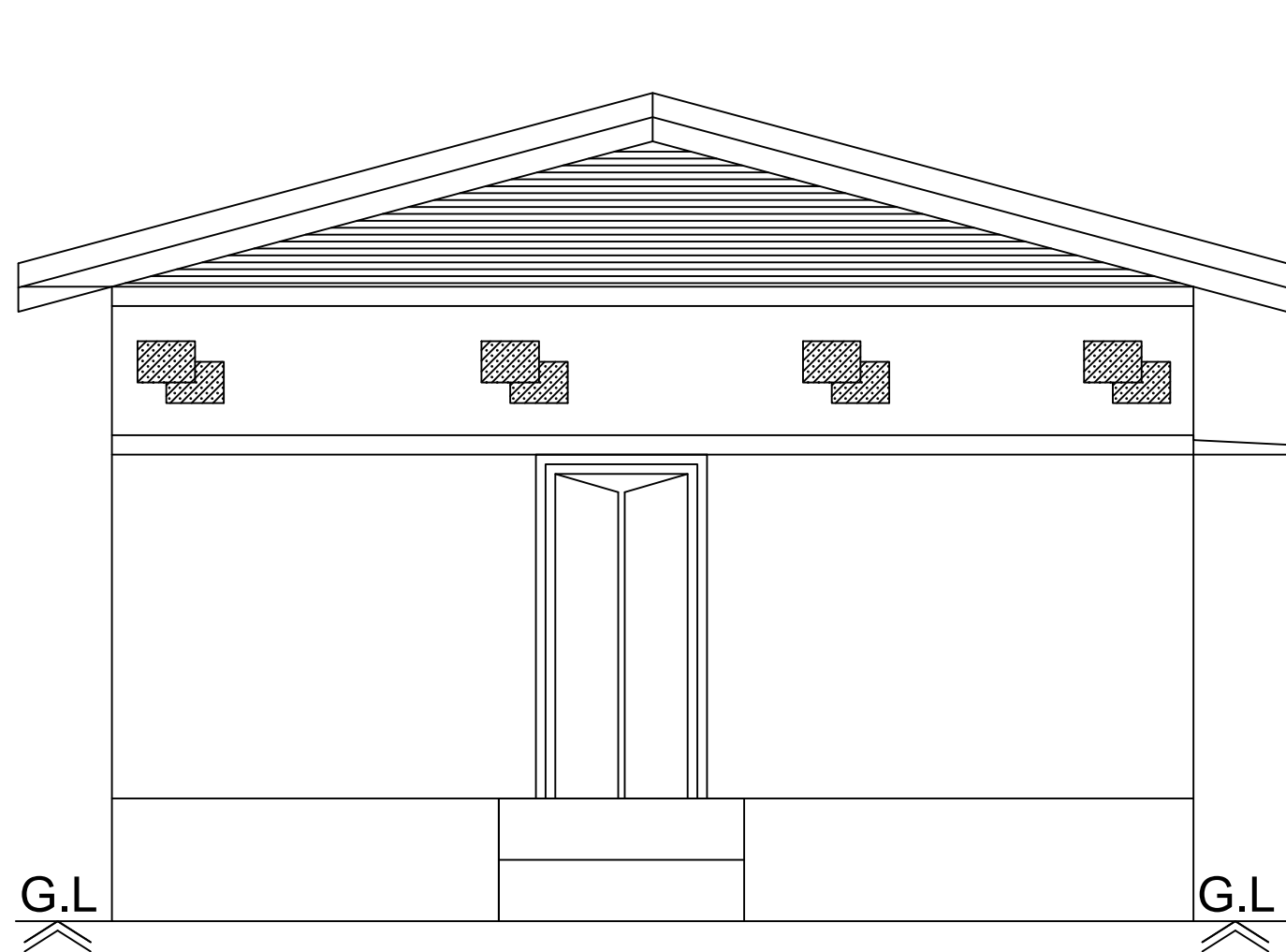
Front Elevation
