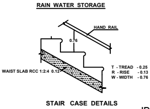
RAIN WATER STORAGE
