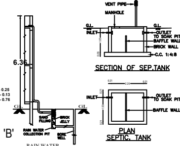
RAIN WATER HARVESTING SYSTEM RWH_CAPACITY_L=1000LTRS
