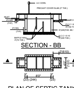
SECTION - BB PLAN OF SEPTIC TANK
