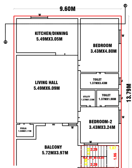
ADY APPROVED FIRST FLOOR PLAN
