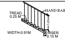
STAIRCASE DETAILS
