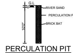
PERCOLATION PIT
