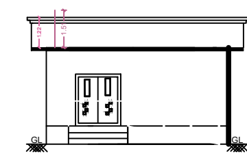
FRONT ELEVATION
