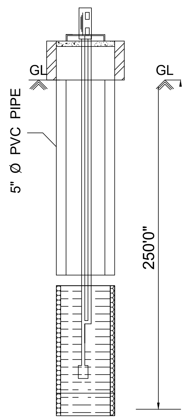
BOREWELL DETAILS
