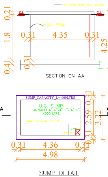
SUMP DETAIL
