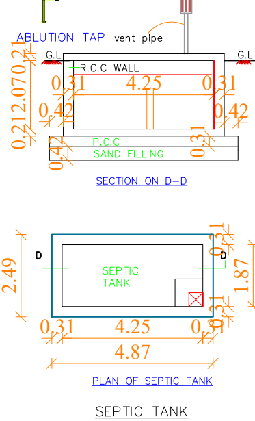
SEPTIC TANK
