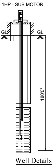
Well Details
