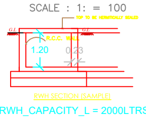
SCALE : 1: = 100 RWK_SECTION (SAMPLE) RWK_CAPACITY_L = 2000LTRS
