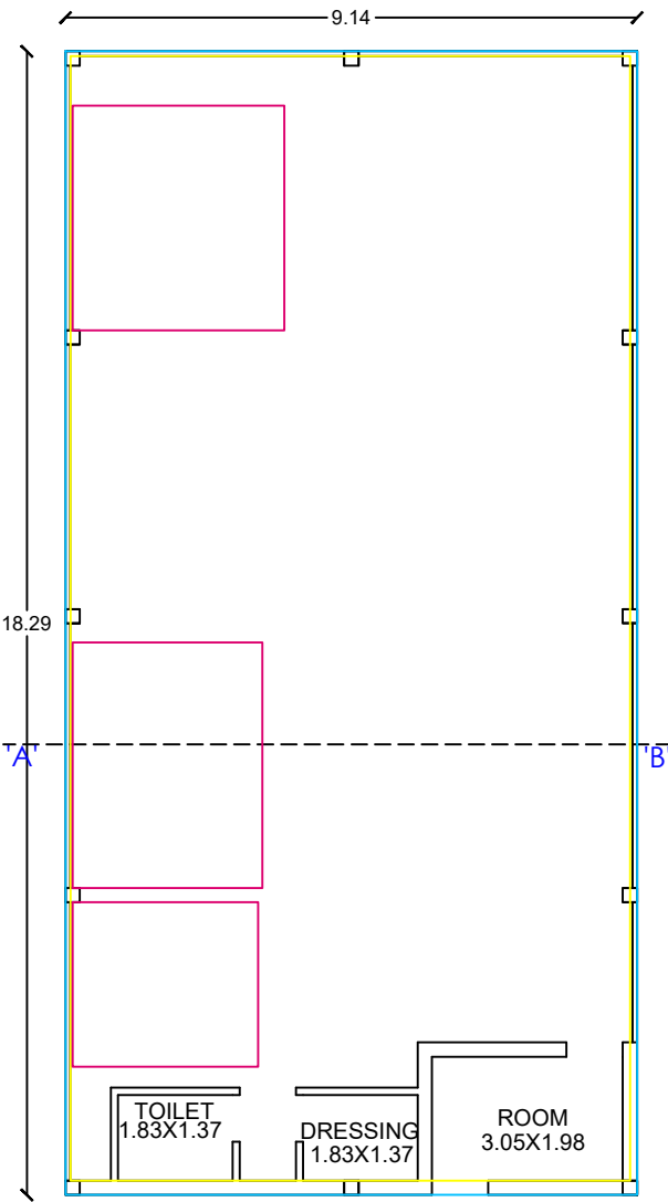
Plan
