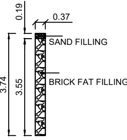
DETAILS OF PERCULATION PIT
