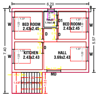
PRO., GROUND FLOOR PLAN
