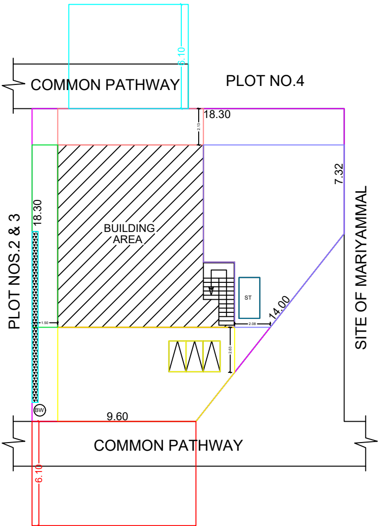
SITE PLAN
