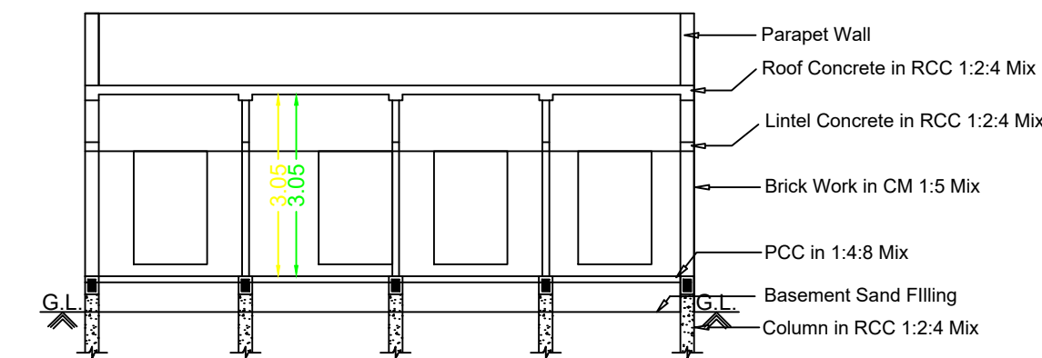
Section RR
