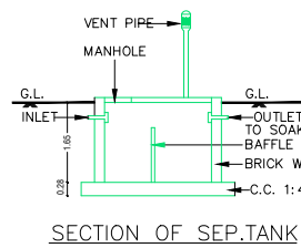
SECTION OF SEP.TANK
