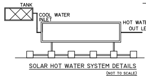
SOLAR HOT WATER SYSTEM DETAILS (NOT TO SCALE)
