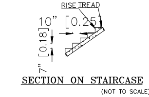
SECTION ON STAIRCASE (NOT TO SCALE)
