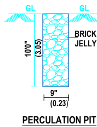
PERCOLATION PIT
