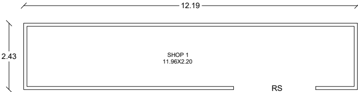
GROUND FLOOR
