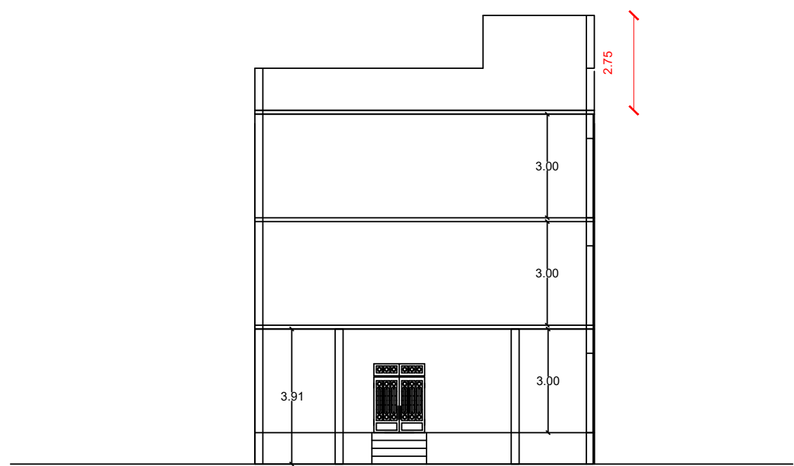
FRONT ELEVATION
