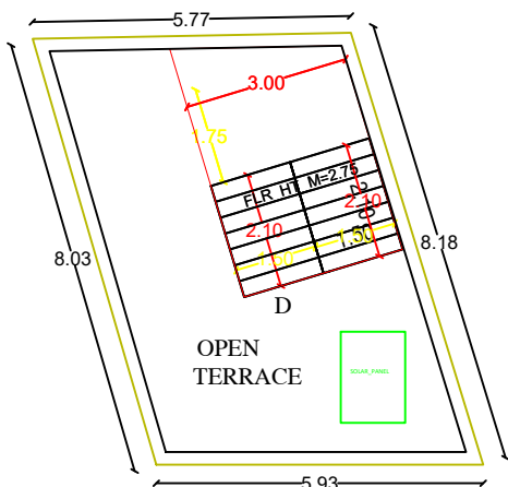
TEREACE FLOOR
