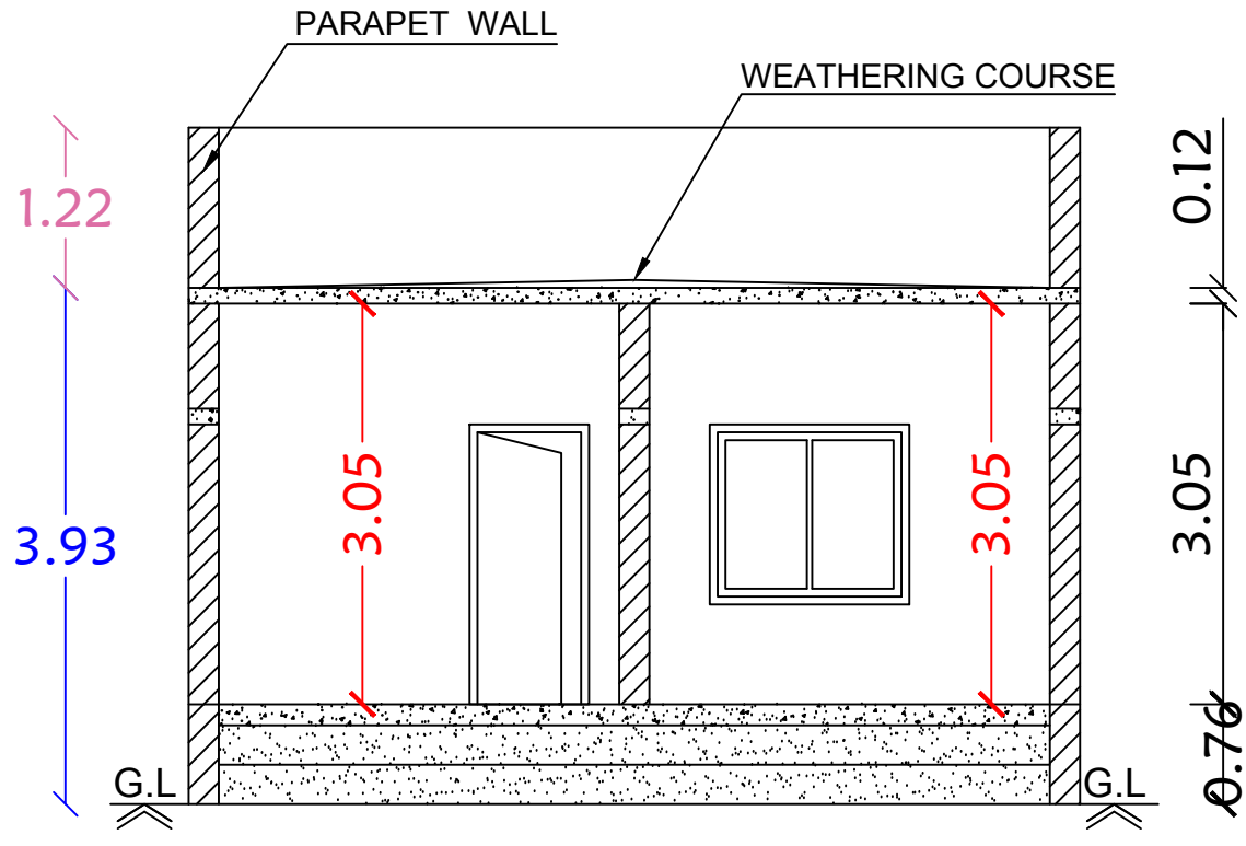
Section on-"AA"
