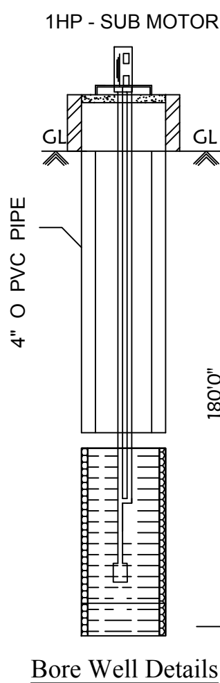
Bore Well Details
