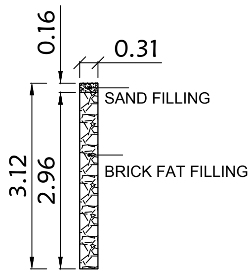
DETAILS OF PERCULATION PIT
