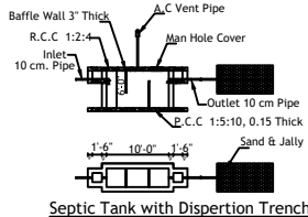
Septic Tank with Dispersion Trench
