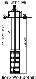
Bore Well Details
