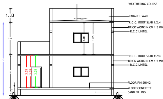
SECTION A1-A1
