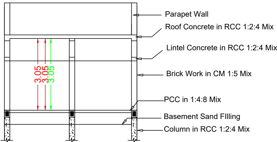
Section RR
