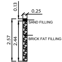
DETAILS OF PERCULATION PIT
