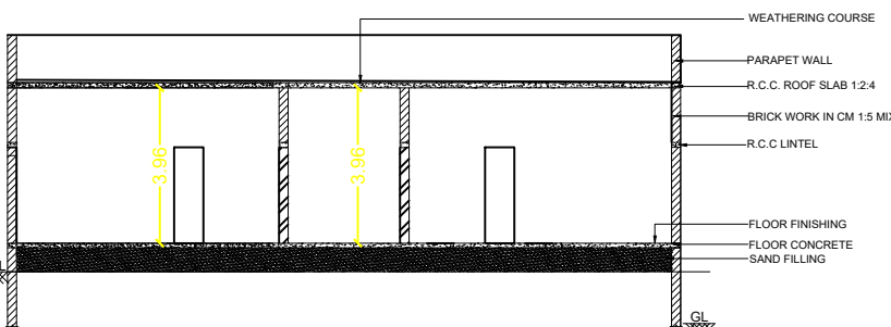
SECTION ON "RI"
