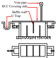
SEPTIC TANK
