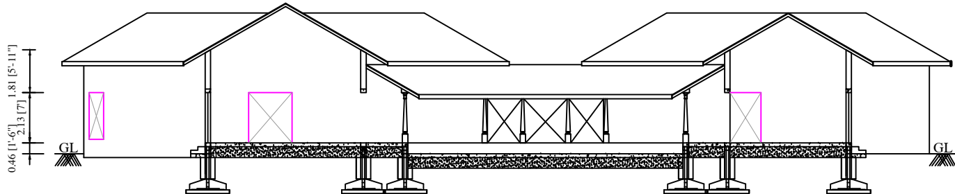
SECTION B-B
