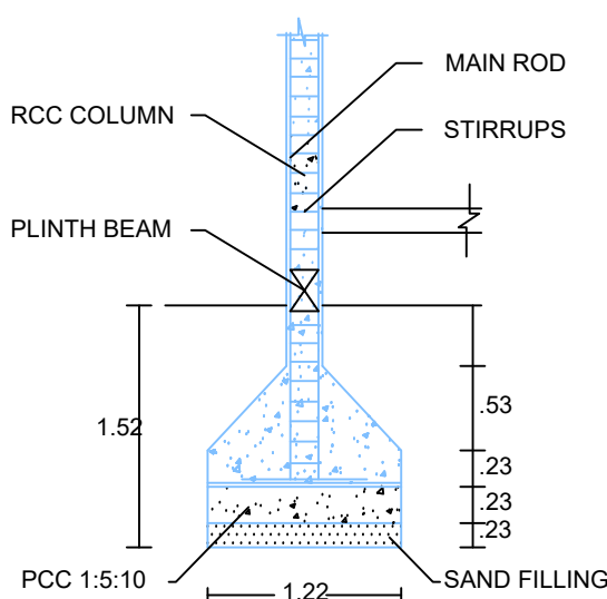
COLUMN DETAILS
