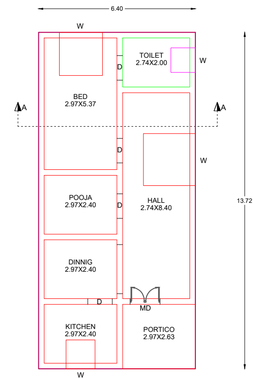
PROPOSED RESIDENTIAL GROUND FLOOR PLAN
