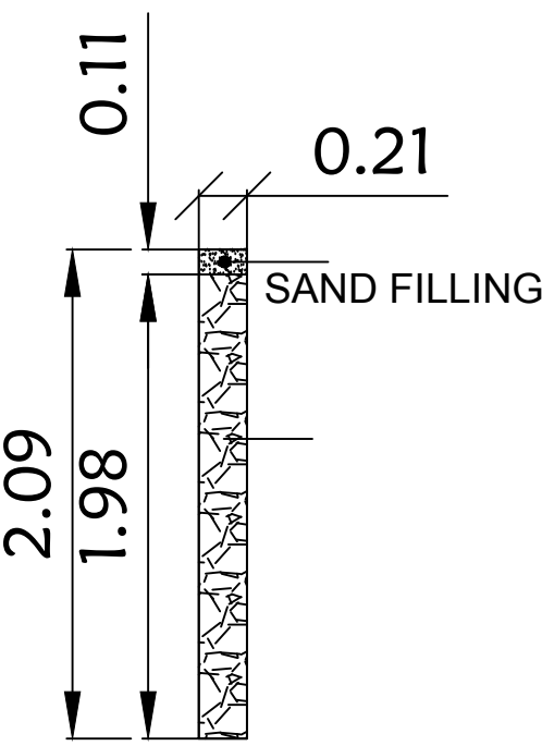
DETAILS OF PERCUATION PIT
