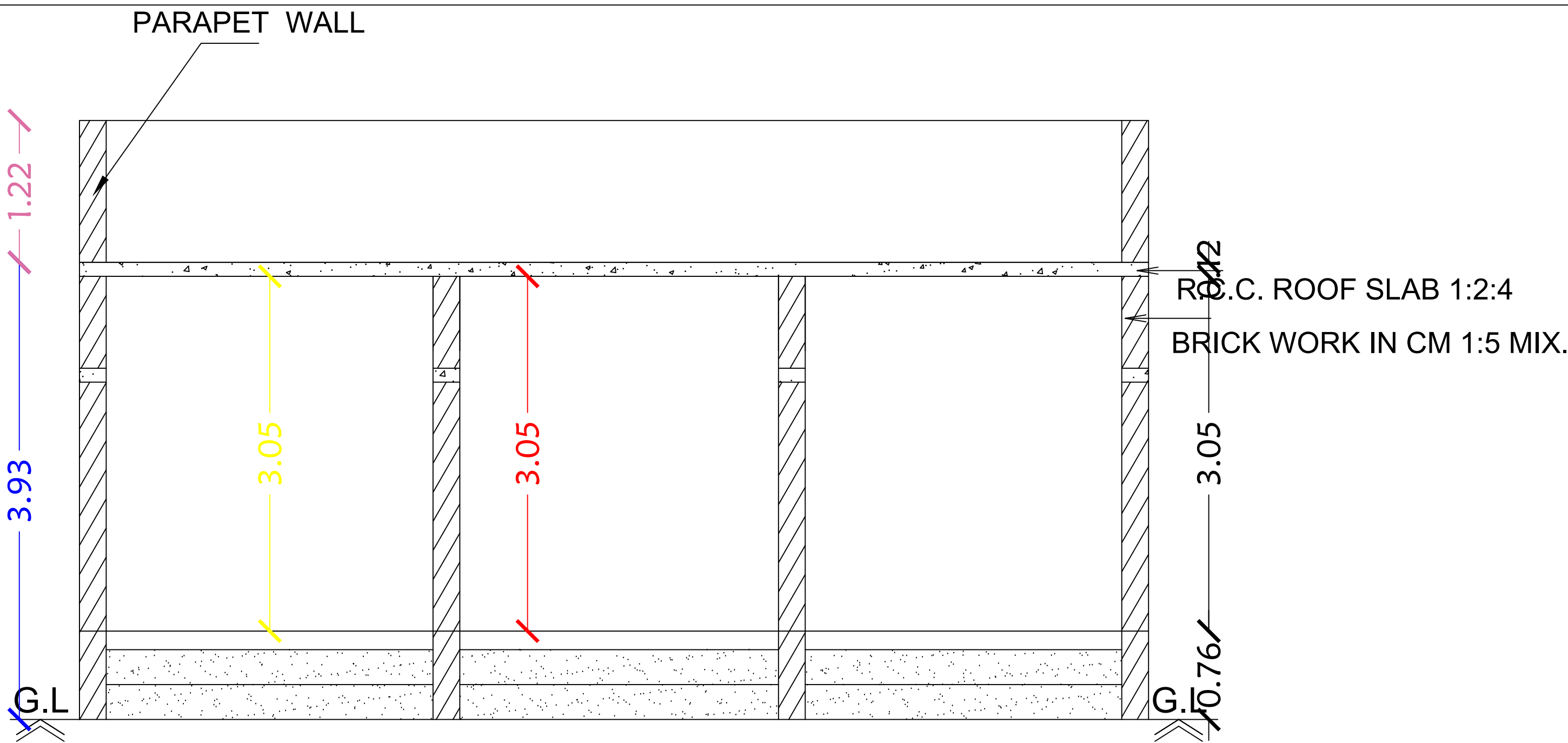
Section on-"AA"
