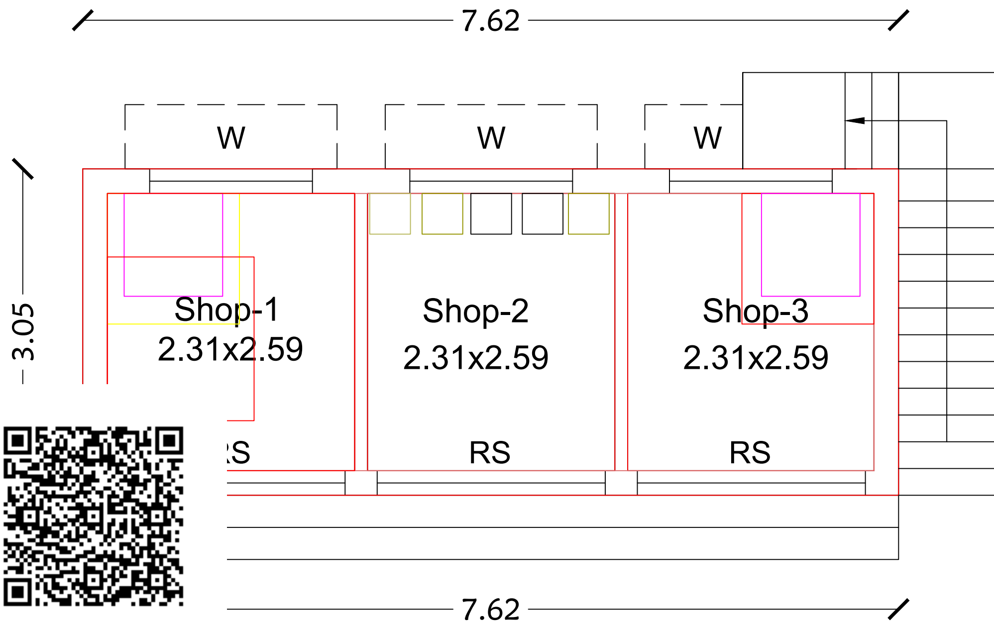
Ground Floor
