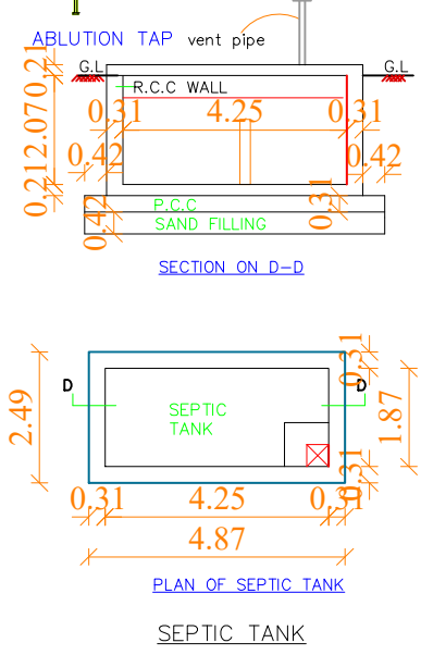
SEPTIC TANK
