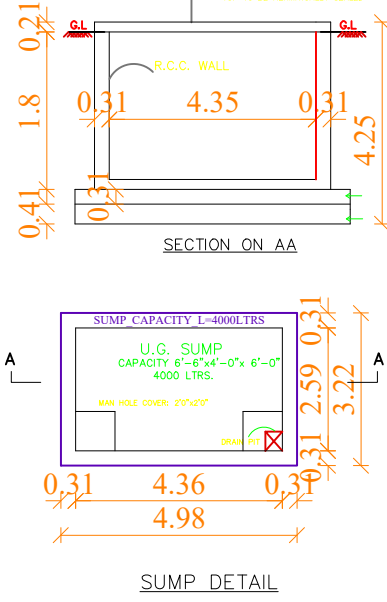
SUMP DETAIL
