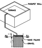
COLLECTION OF SUMP RAINWATER HARVESTING FROM TERRACE
