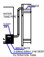
RAIN WATER
