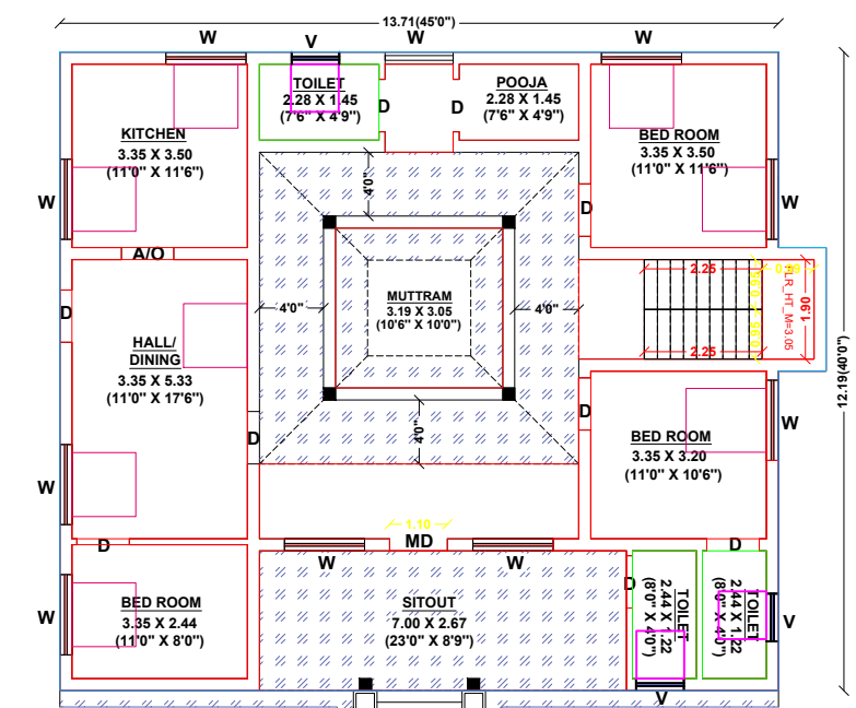
FLOOR-GROUND PLAN
