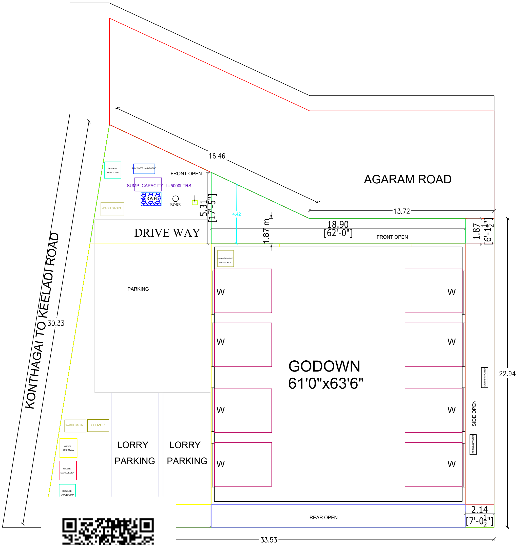
RO.GROUND FLOOR PLAN
