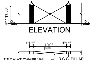
COMPOUND WALL PLAN
