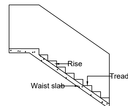
DETAIL OF STAIRCASE
