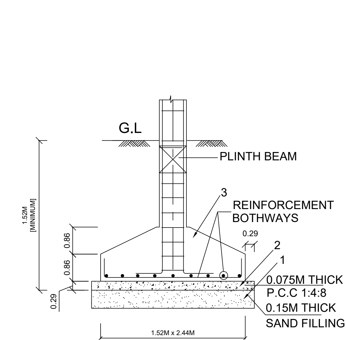
FRONT ELEVATION
