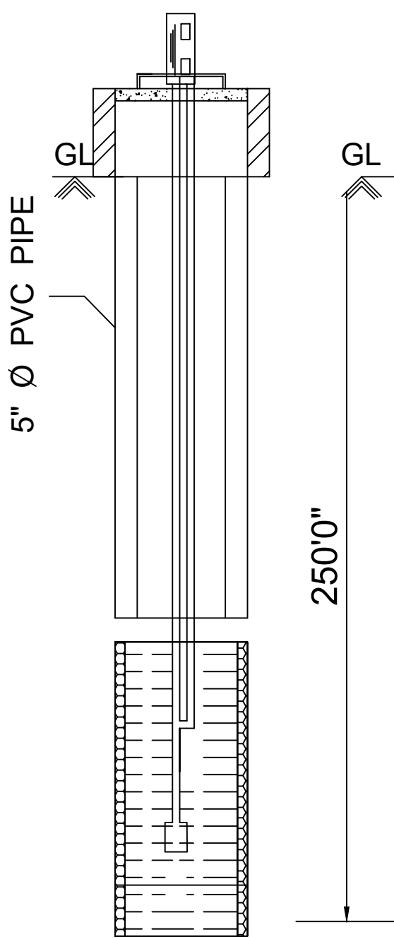
BOREWELL DETAILS
