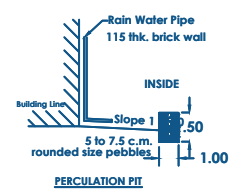
PERCOLATION PIT
