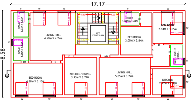
PROPOSED SECOND FLOOR PLAN
