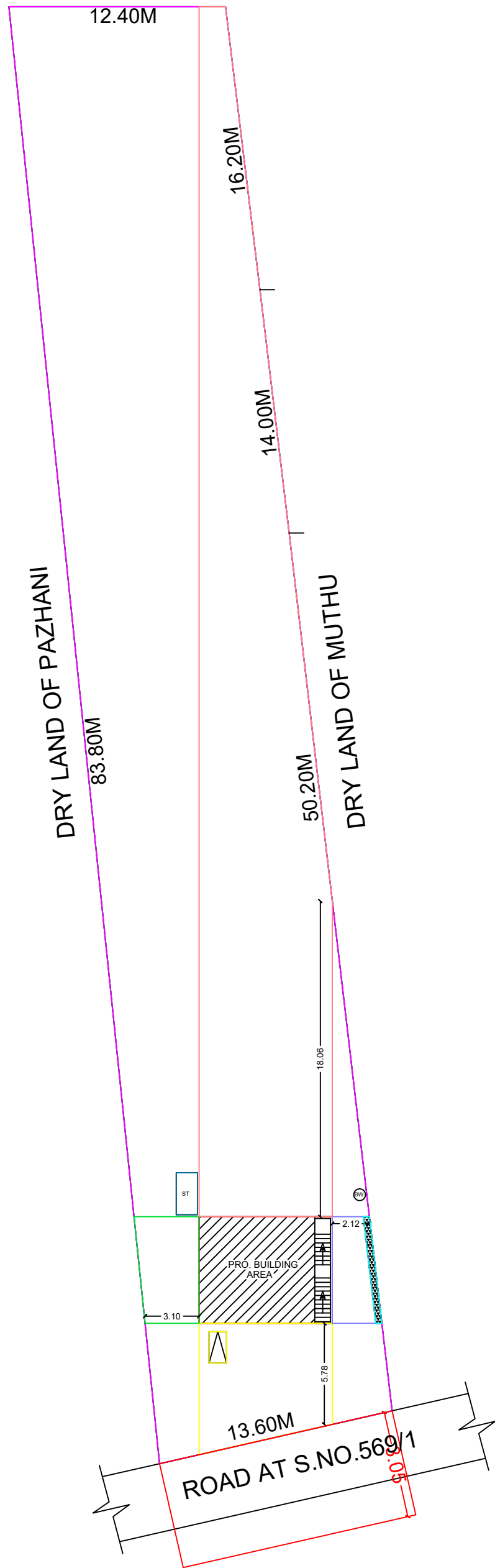
SITE PLAN
