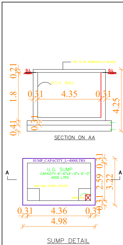
SUMP DETAIL
