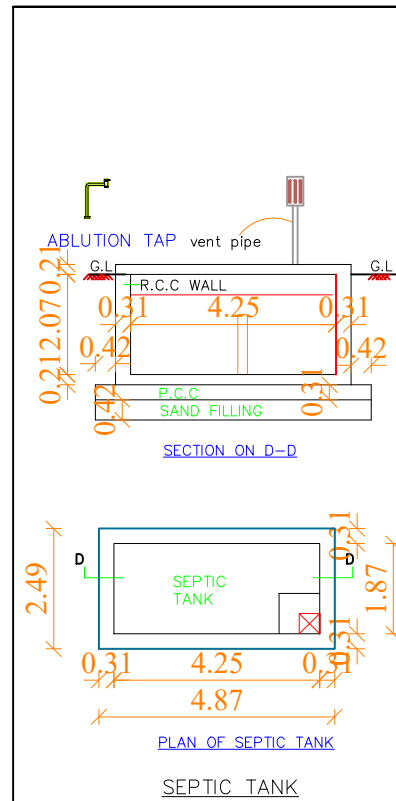
SEPTIC TANK
