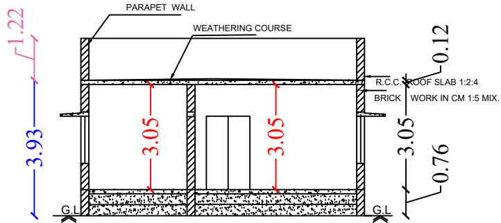
Section on-"AA"
