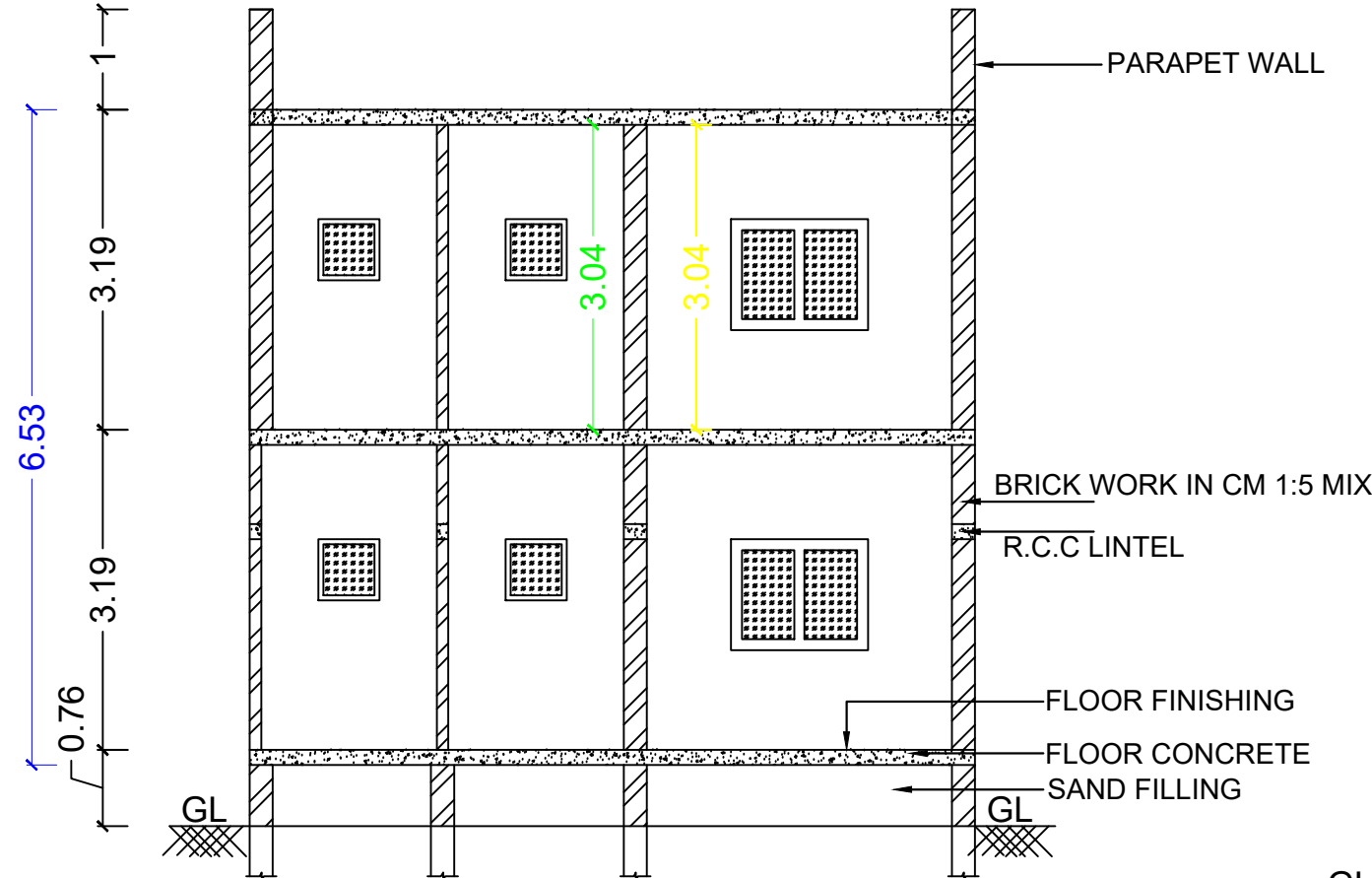
SECTION AT A1-A1
