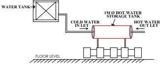
Solar Hot Water System Detail
