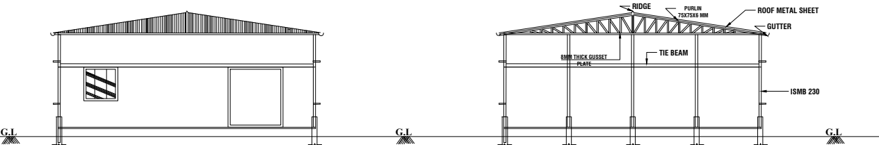
FRONT ELEVATION
