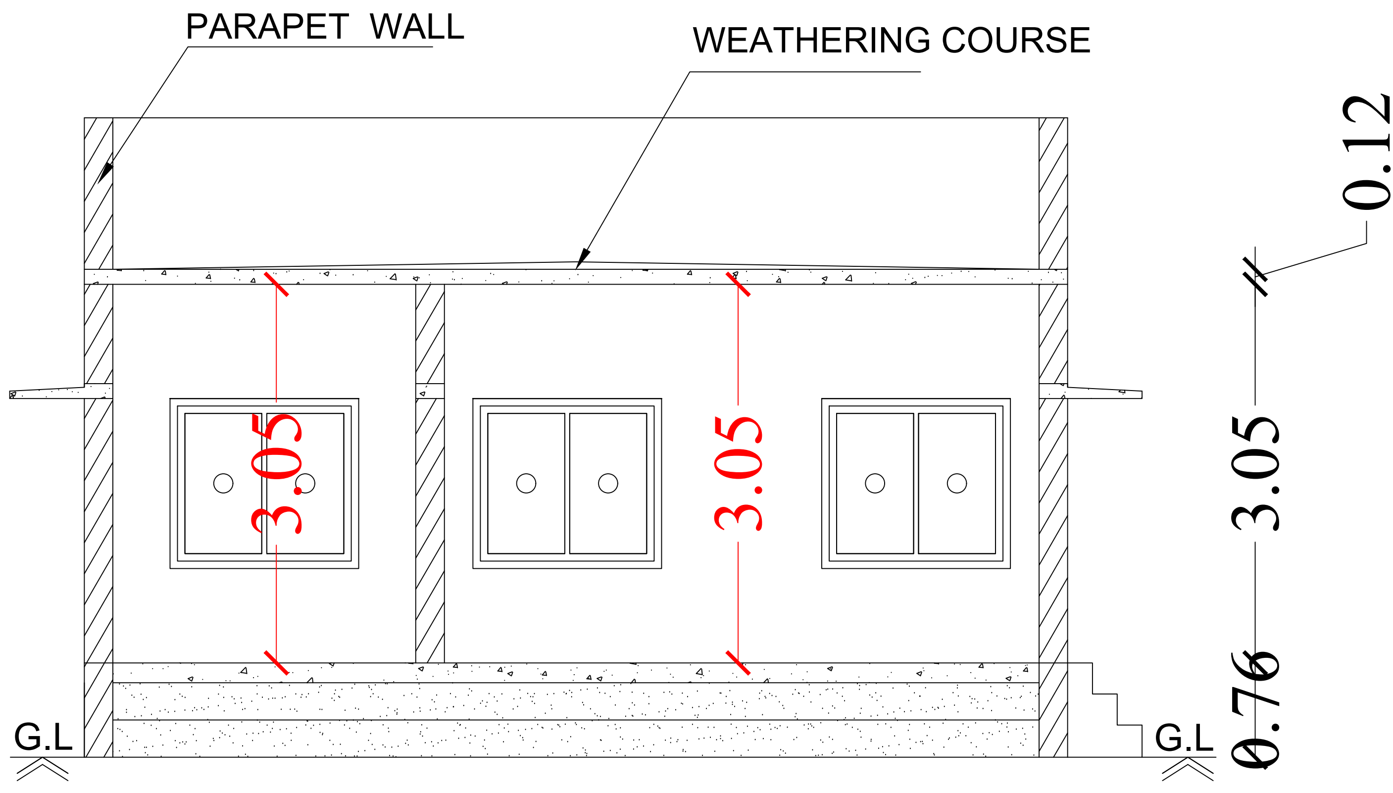
Section on-"AA"
