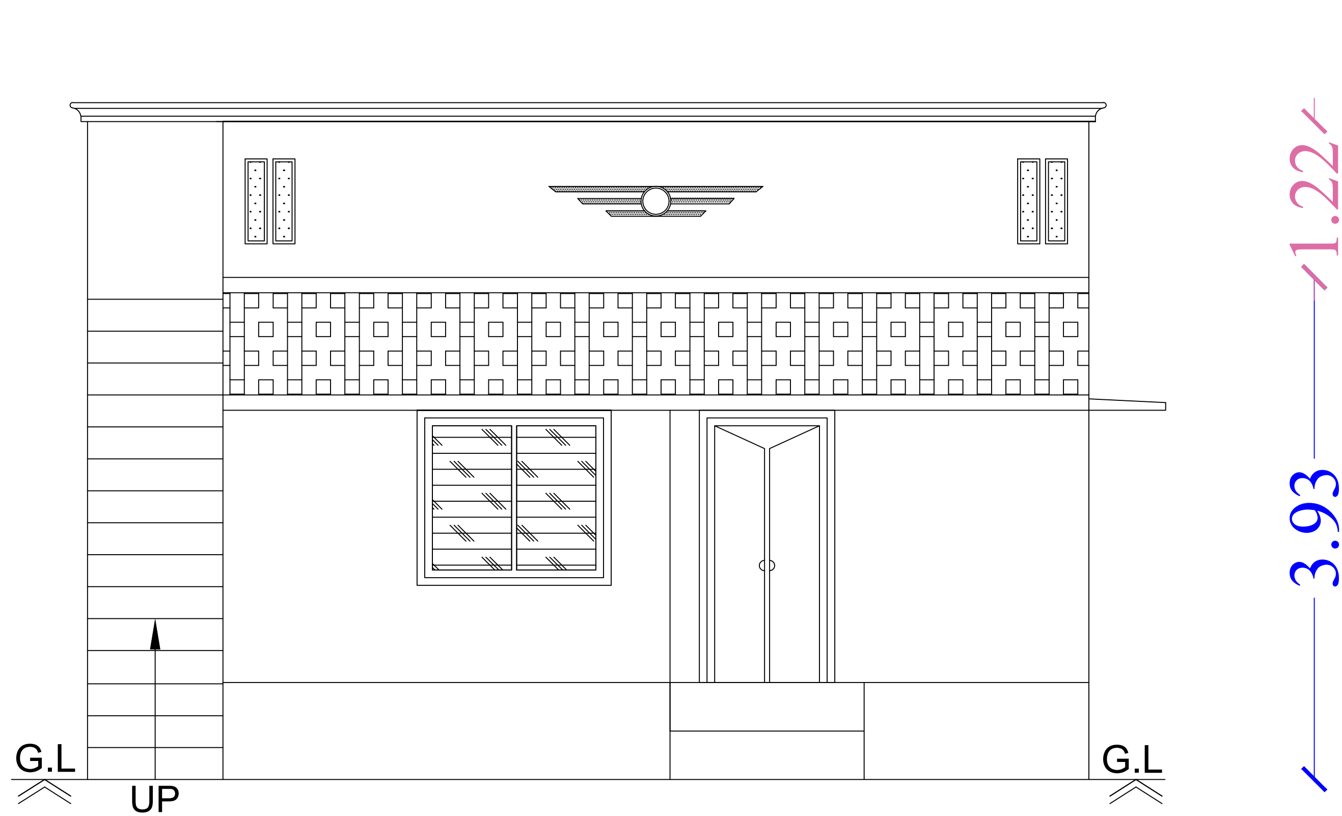
Front Elevation
