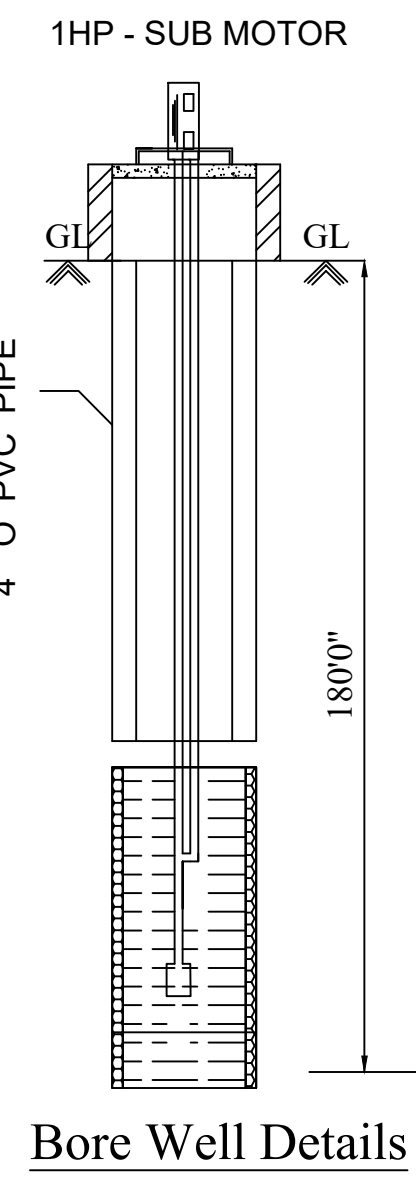
Bore Well Details
