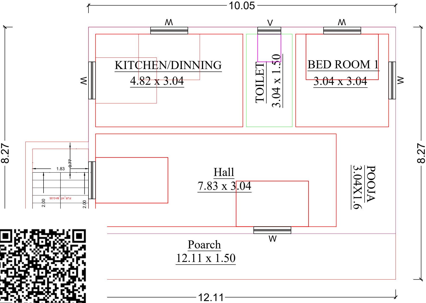
ROUND FLOOR PLAN
