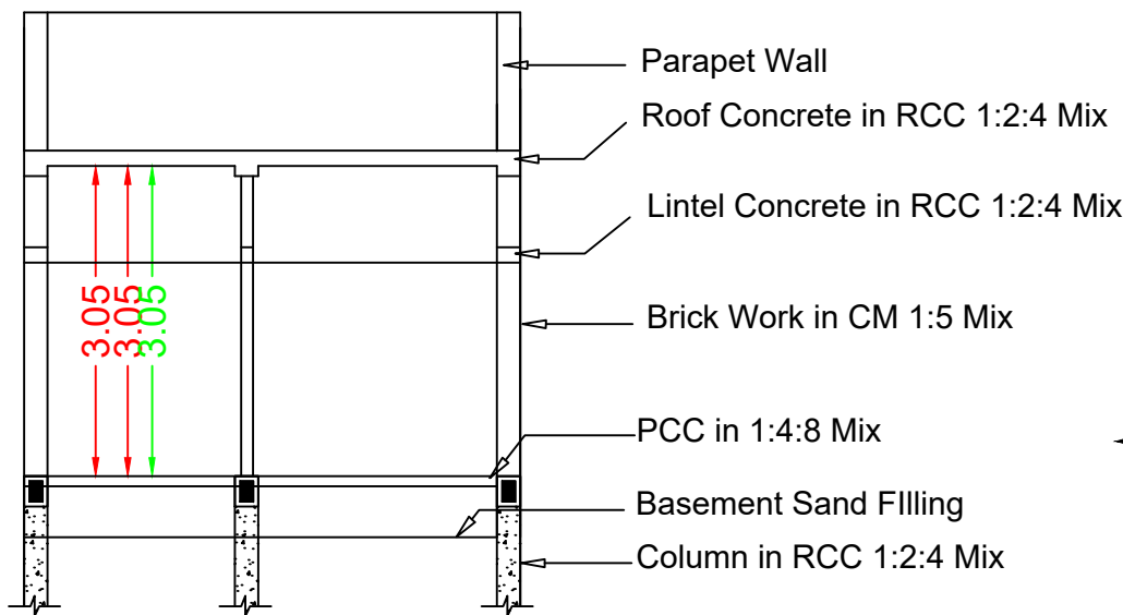
Section RR
