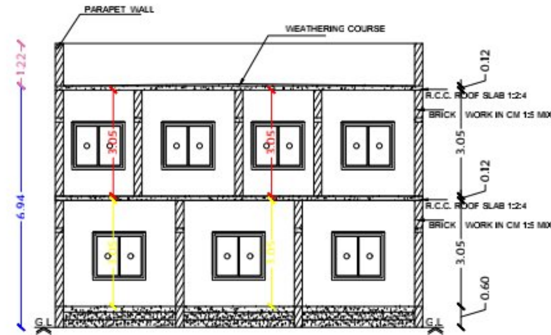
Section on-"AA"
