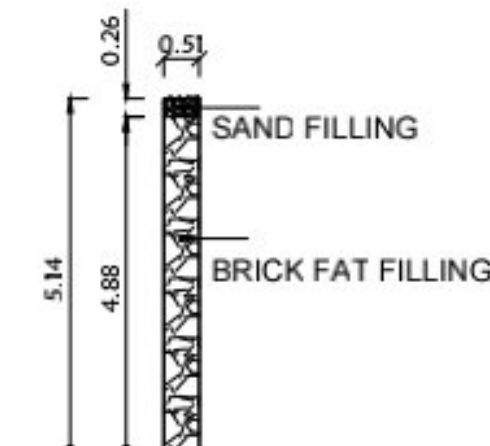
DETAILS OF PERCOLATION PIT
