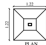
FOUNDATION DETAILS
