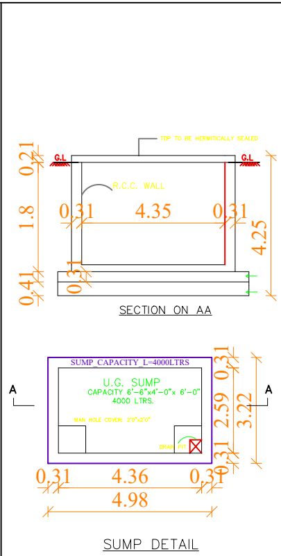
SUMP DETAIL
