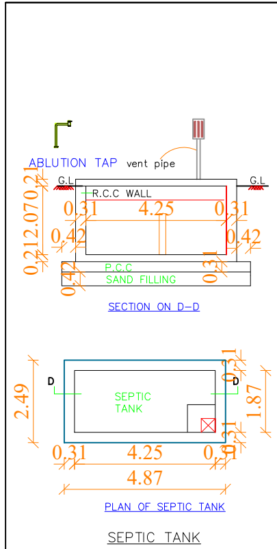
SEPTIC TANK
