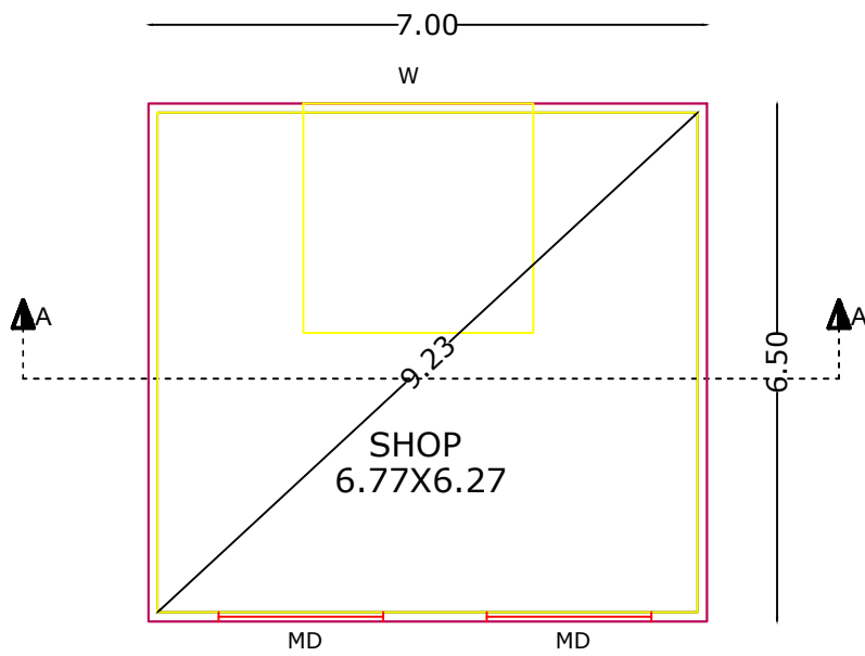
PROPOSED COMMERCIAL ND FLOOR PLAN
