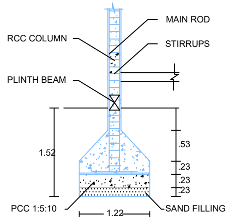
COLUMN DETAILS
