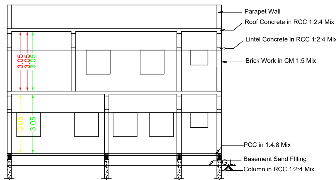
Section RR
